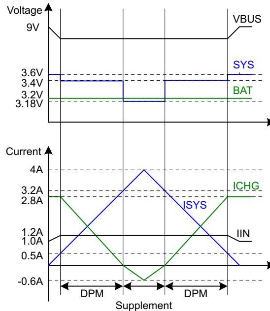
Figure 17. DPM Response
