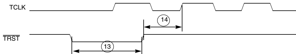
Figure 17. \overline{TRST} Timing
