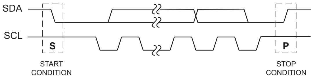
Figure 7. Bit Transfer
