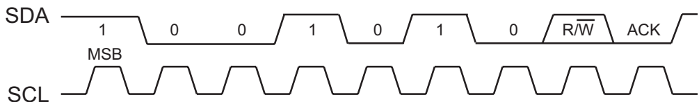
Figure 9. Slave Address
