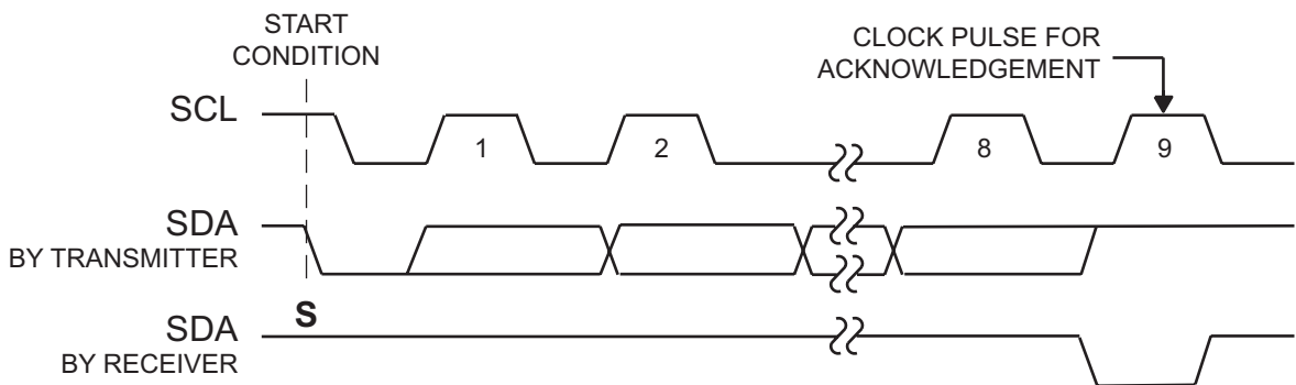
Figure 8. Acknowledge
