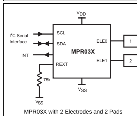
Figure 1. Pin Connections
