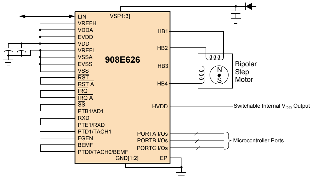
Figure 1. 908E626 Simplified Application Diagram
