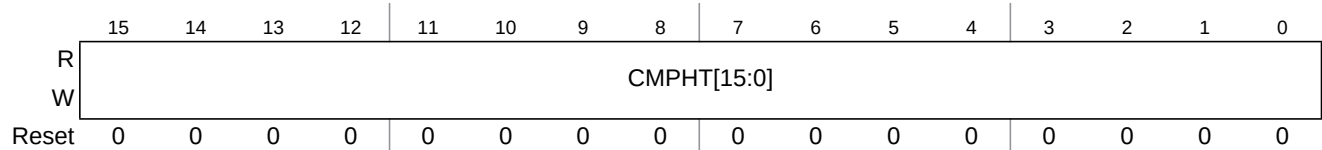
Figure 10-13. ATD Compare Higher Than Register (ATDCMPHT)
