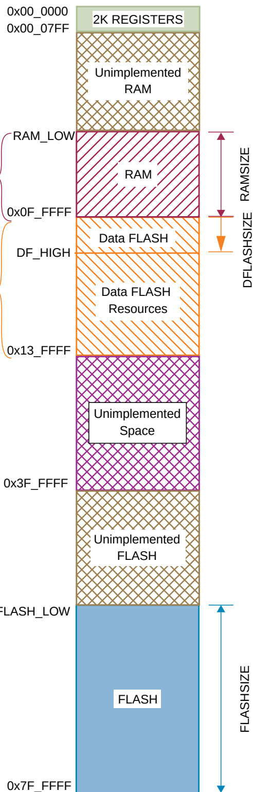
Figure 3-19. S12X CPU &amp; BDM Global Address Mapping
