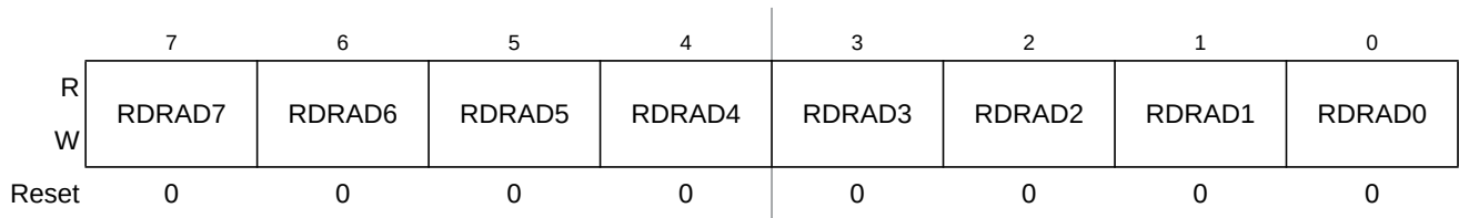
Figure 2-22. Port AD Reduced Drive Register (RDRAD)
