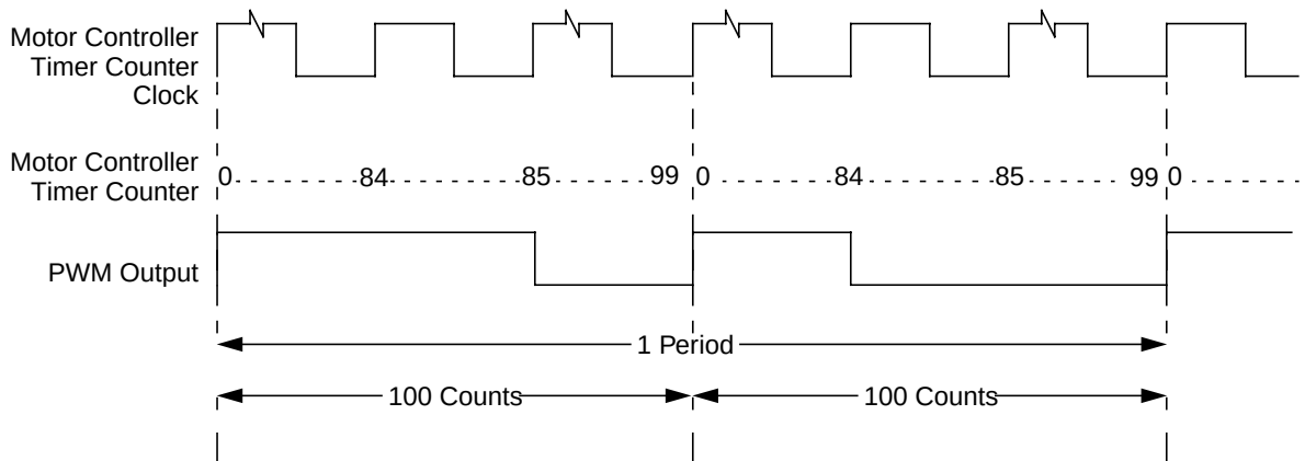
Figure 11-20. PWM Output: DITH = 1, MCAM[1:0] = 10, MDCD = 31, MCPER = 200, RECIRC = 0
