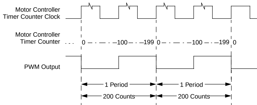
Figure 11-17. PWM Output: DITH = 0, MCAM[1:0] = 01, MCDL = 100, MCPER = 200, RECIRC = 0
