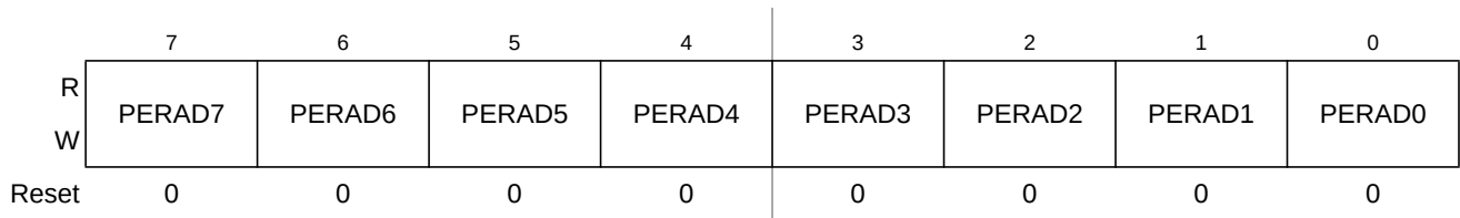
Figure 2-23. Port AD Pull Device Enable Register (PERAD)
