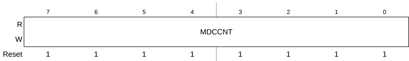
Figure 12-7. Modulus Down-Counter Count Register Low (MDCCNT)
