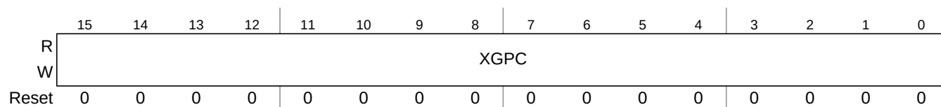
Figure 5-10. XGATE Program Counter Register (XGPC)
