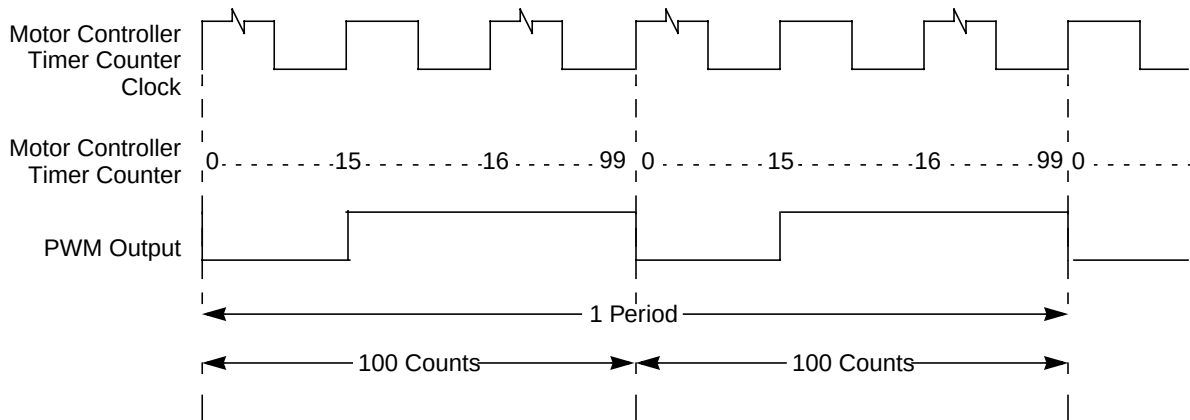
Figure 11-19. PWM Output: DITH = 1, MCAM[1:0] = 01, MDCD = 30, MCPER = 200, RECIRC = 0
