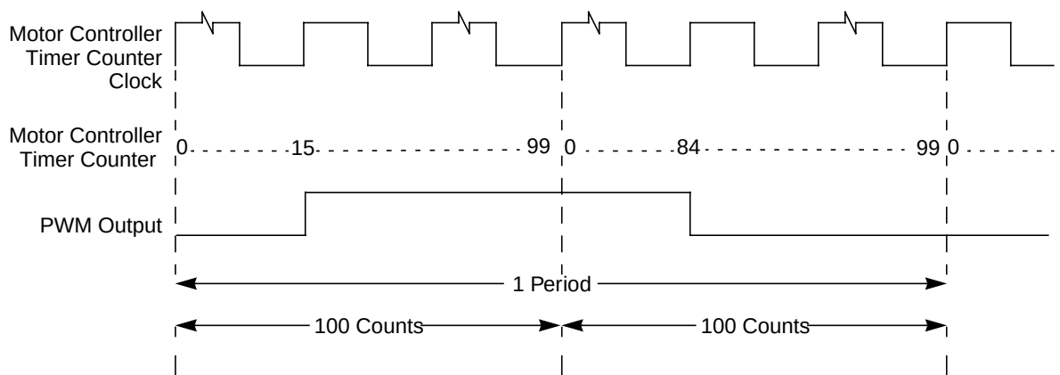
Figure 11-21. PWM Output: DITH = 1, MCAM[1:0] = 11, MDCD = 31, MCPER = 200, RECIRC = 0
