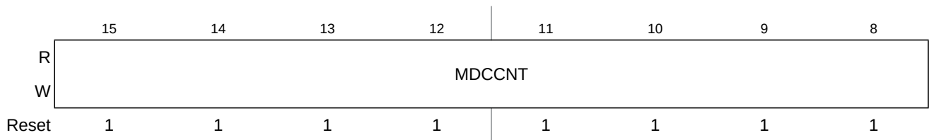
Figure 12-6. Modulus Down-Counter Count Register High (MDCCNT)
