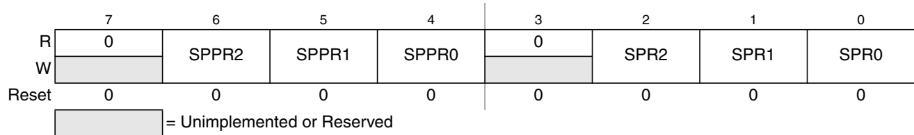
Figure 21-5. SPI Baud Rate Register (SPIBR)
