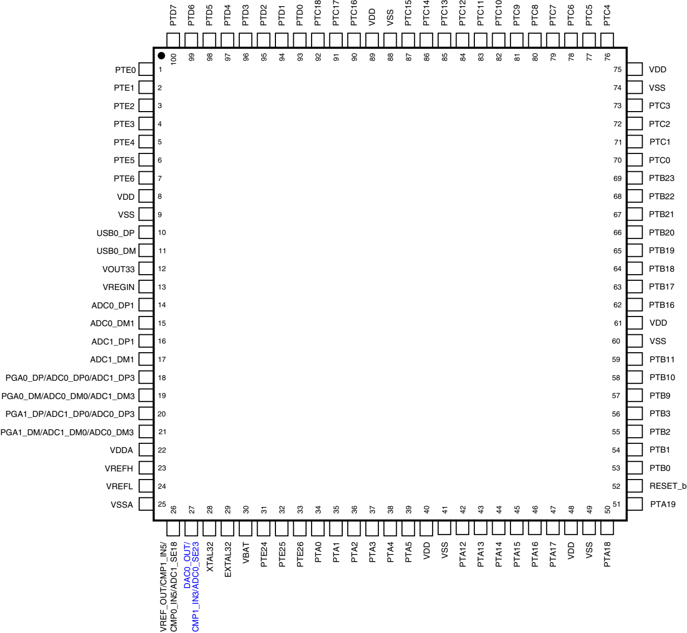
Figure 29. K20 100 LQFP Pinout Diagram
