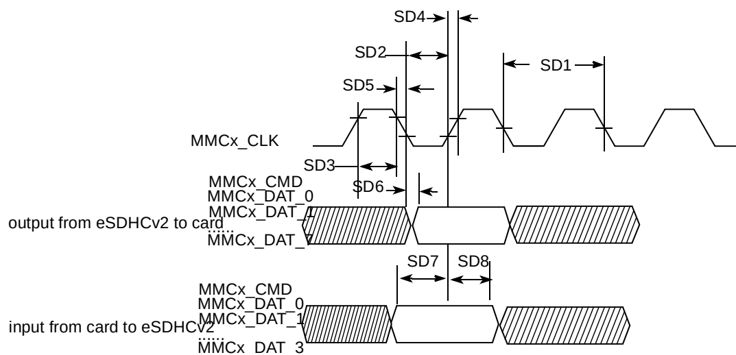
Figure 41. eSDHCv2 Timing
